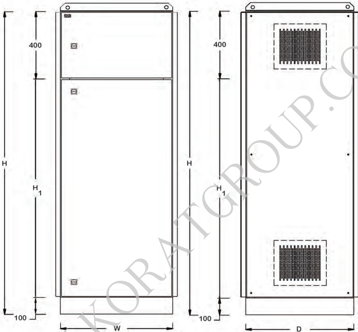
FRONT VIEW
